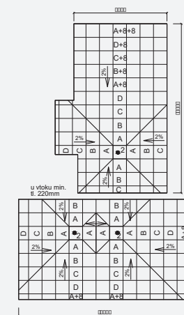
Design of flat roof pitches - 2%
