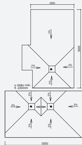
Design of flat roof pitches - 2%
